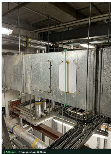
Duct height (mm): measuring photo
